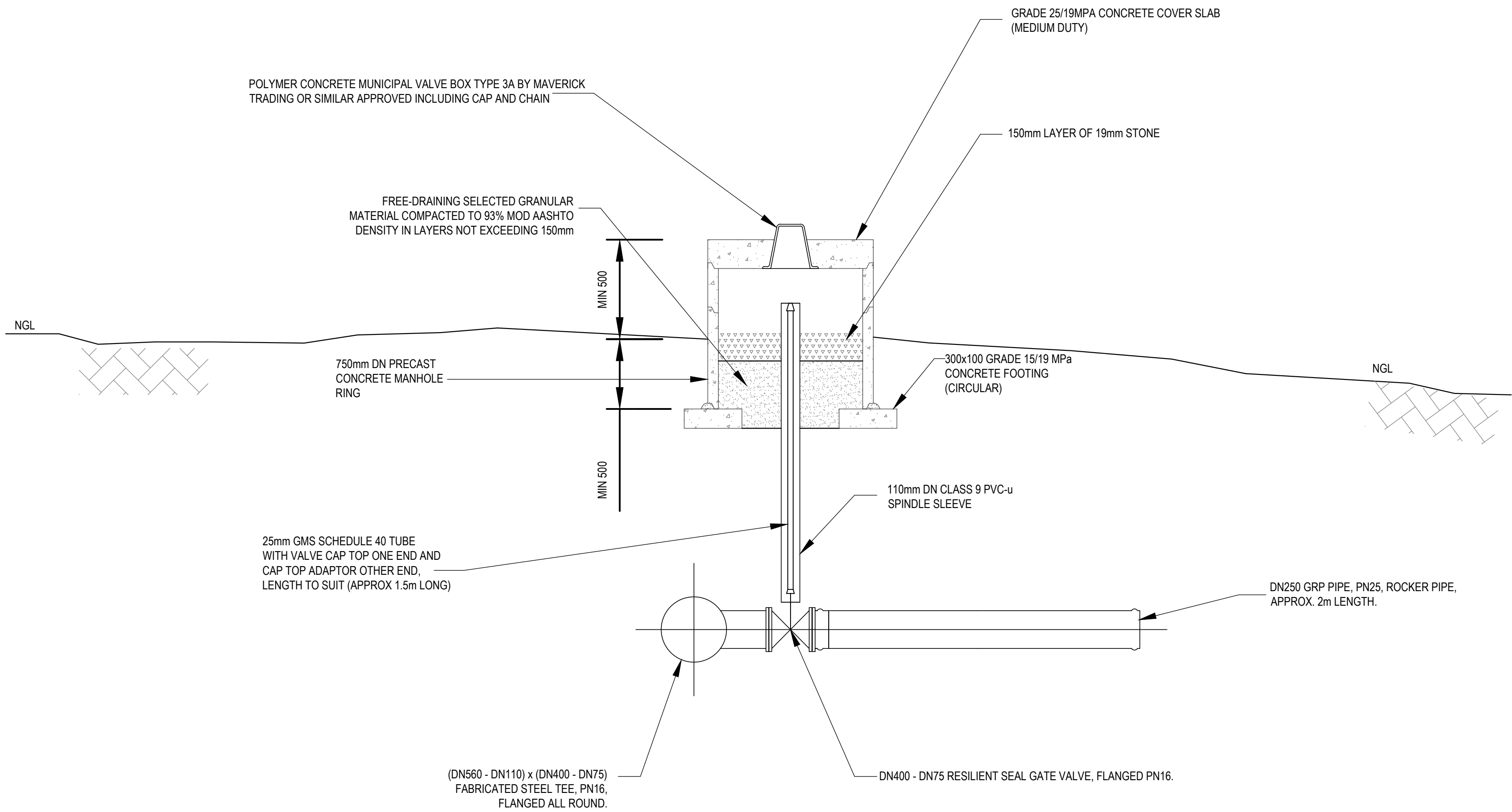
OFF TAKE DETAIL: MH SECTION N.T.S.
