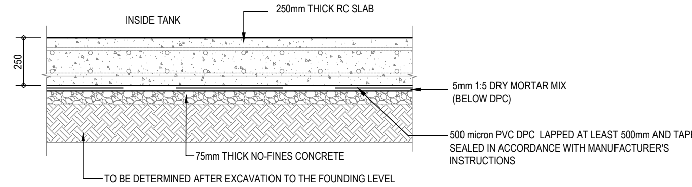
TYPICAL FLOOR DETAIL SCALE 1:20
