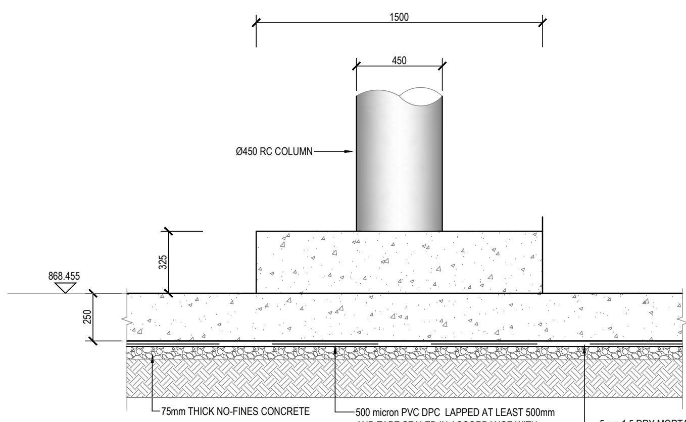
TYPICAL SECTION THROUGH RC COLUMN AND BASE SCALE 1:20
