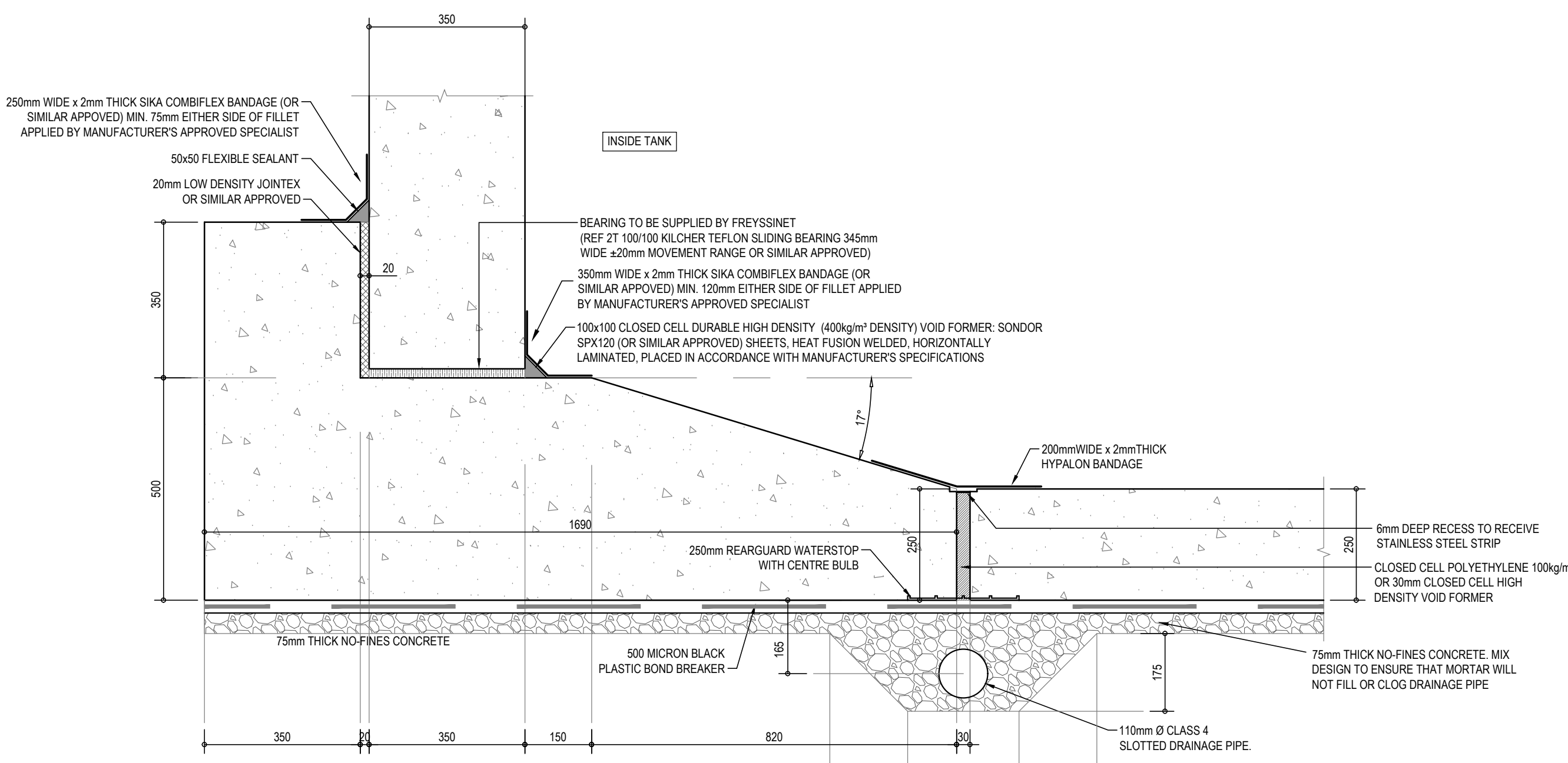
DETAILED SECTION 01 THROUGH FOOTING WITH EXPANSION JOINT SCALE 1:10
