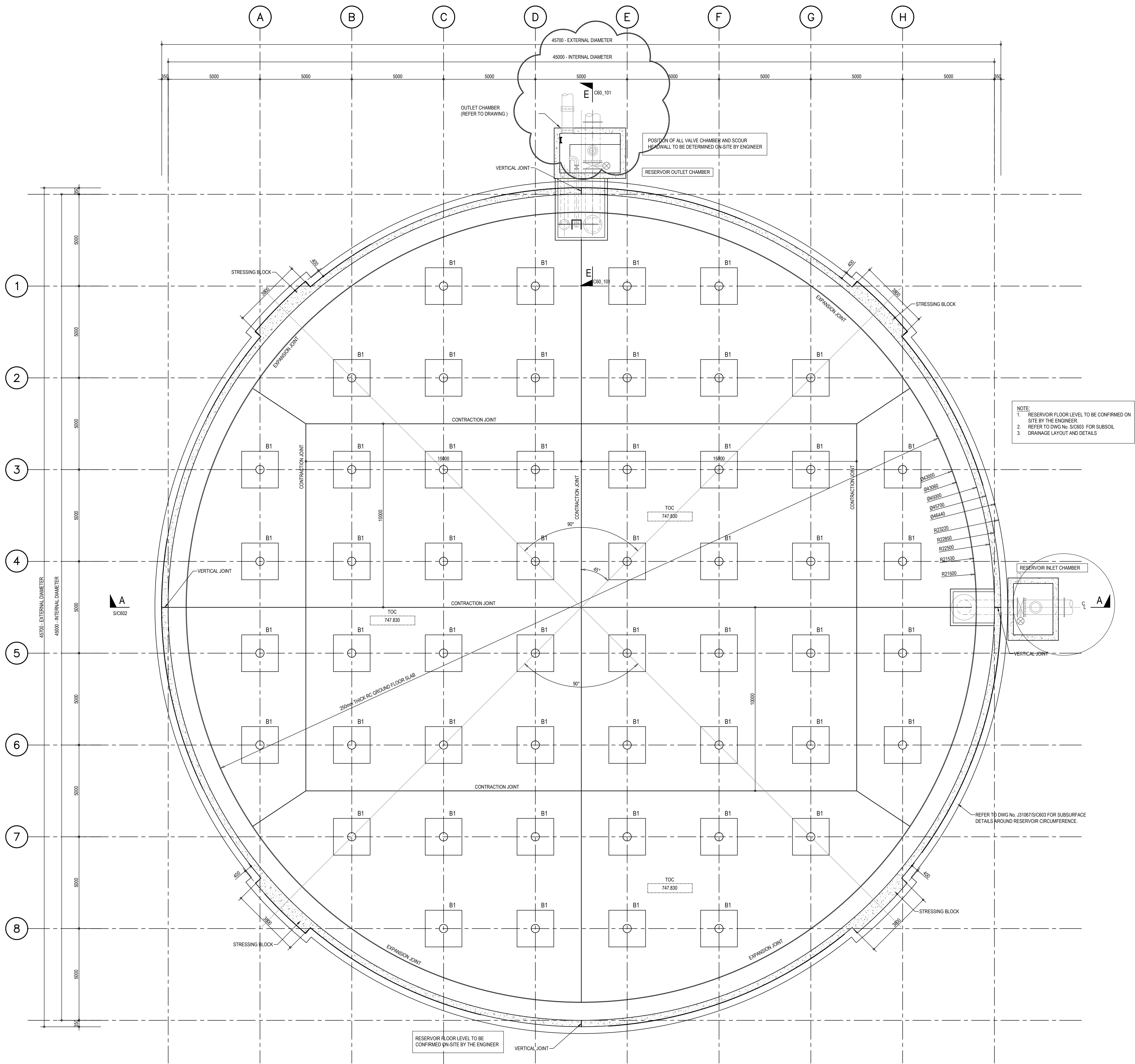
FLOOR LAYOUT PLAN SCALE 1:100
